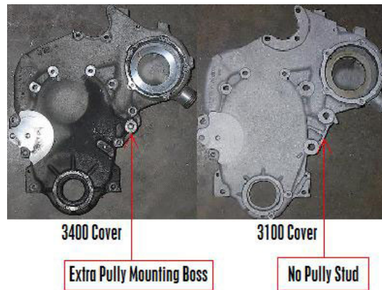
3100 Timing Chain Cover w/Extra Knob Location Pointed Out
