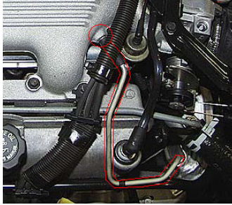
The Modulator Vacuum line on the 3.1.
